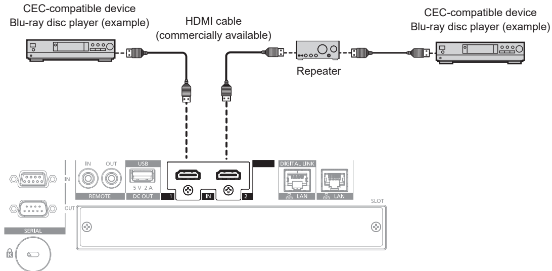
Connection example with CEC-compatible device
